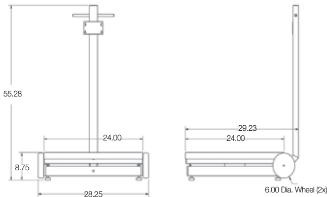
Wheel Model
