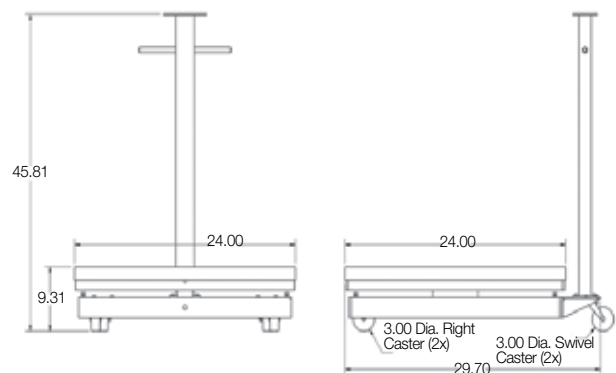
Caster Model
